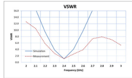
Figure 9. Comparison between Simulation and Measurement Result of VSWR
