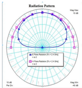
Figure 11. Radiation Pattern of Fractal Microstrip Antenna
