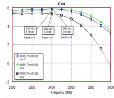
Figure 12. Gain of Fractal Microstrip Antenna
