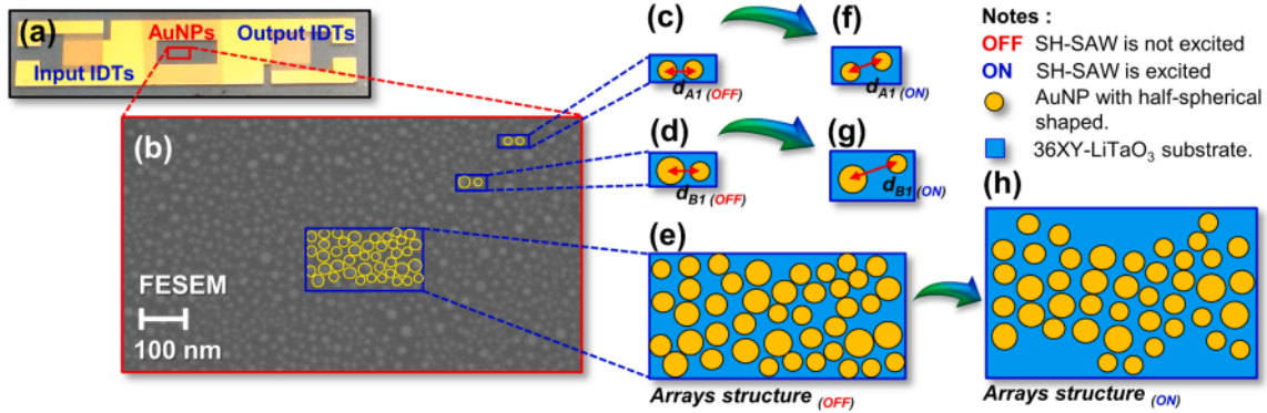
Fig. 5. (a) A fabrication of the proposed device including the structure of input/output IDTs and arrays AuNPs on 36XY-LiTaO 3 substrate, (b) the 2D morphology image of the arrays AuNPs on the propagation surface of the SH-SAW device using FE-SEM. Reproducing the morphological AuNPs structure to (c) identical dimer AuNPs, (d) nonidentical dimer AuNPs, and (e) arrays AuNPs structure for OFF-condition. The AuNPs structure with ON-condition for (f) identical dimer AuNPs, (g) nonidentical dimer AuNPs, and (h) arrays AuNPs for ON-condition.
