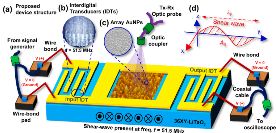
Fig. 1. (a) A proposed device structure of reconfigurable LSPR spectrum based on acousto-dynamic coupling array AuNPs induced by shear horizontal vibration, (b) Interdigital transducers were designed at frequency of 51.5 MHz, (c) 2D-SEM image of array AuNPs on the propagation surface of SH-SAW, (d) the shear-horizontal surface acoustic waves excited on a 36XY-LiTaO 3 substrate after applying an electric signal via interdigital transducers.
