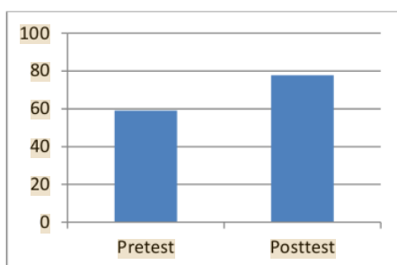
Diagram 3. Result Score of Pretest and Posttest
