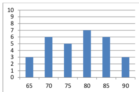
Diagram 2. Result of Score Posttest
