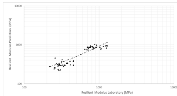
Figure 8. Comparison of laboratory and prediction model.
