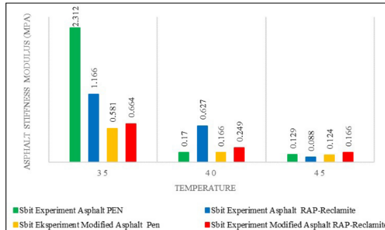
Figure 5. Asphalt stiffness modulus.
