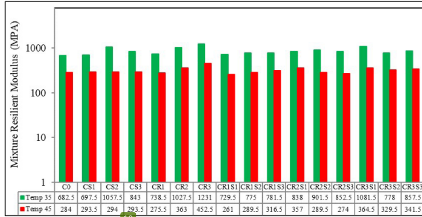
Figure 6. Mixture Resilient Modulus.
