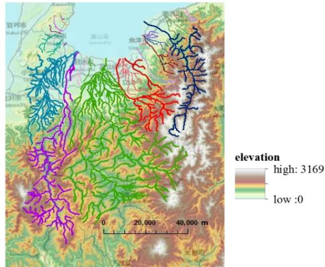
Figure 2. DEM (J-FlowDir) around study area
