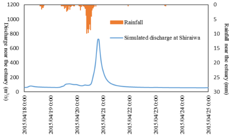
Figure 6. Simulated discharge at Shiraiwa river using model parameters
