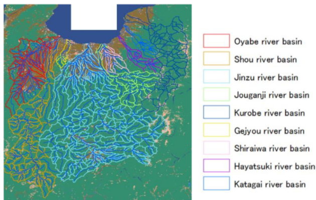
Figure7. 9 river basins in comparison
