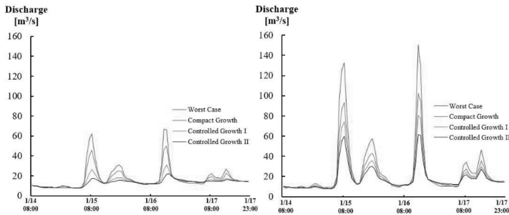
Fig. 4 Simulated river discharge [m 3 /s] of each scenario at Katulampa Station in 2020 and 2050
