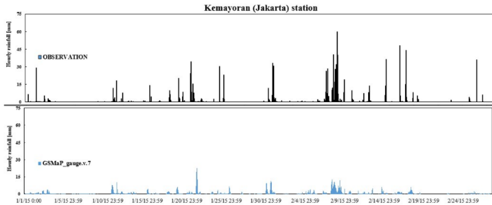
Fig. 2 Comparison of hourly precipitation between GSMaP gauge.v7 and observation
