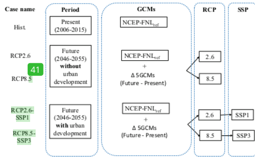
Fig. 4. Experiment cases.
