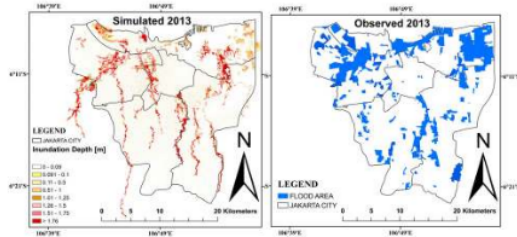
Fig. 5. Comparison of the simulated (left) and observed (right) inundation areas [15].
