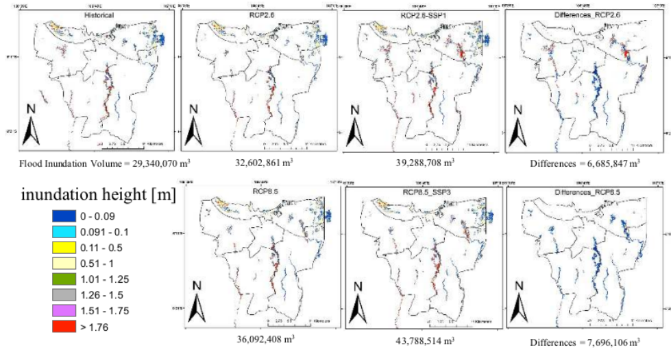
Fig. 10. Comparison of the simulated 10 years averaged maximum flood inundation depths in each scenario and the differences of w/w SSPs.
