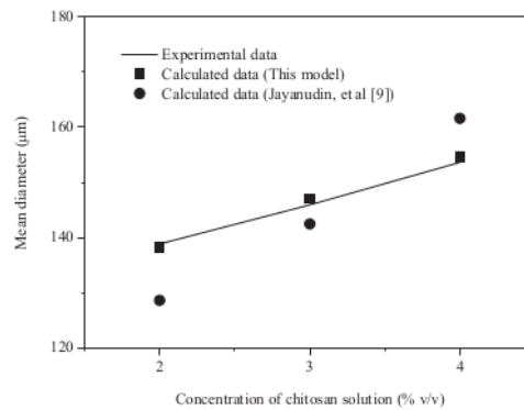
FIGURE 4. Comparison of empirical equation of dimensionless numbers that is conducted to predict diameter of microcapsules from this study with the result that is reported by Jayanudin, et al [9]
