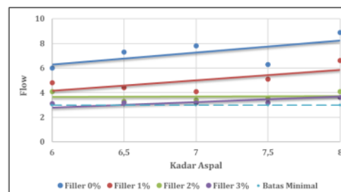
Gambar 6. Perbandingan Nilai Flow
