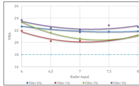
Gambar 2. Perbandingan Nilai VMA
