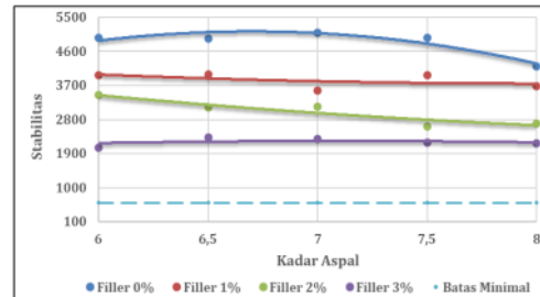
Gambar 5. Perbandingan Nilai Stabilitas
