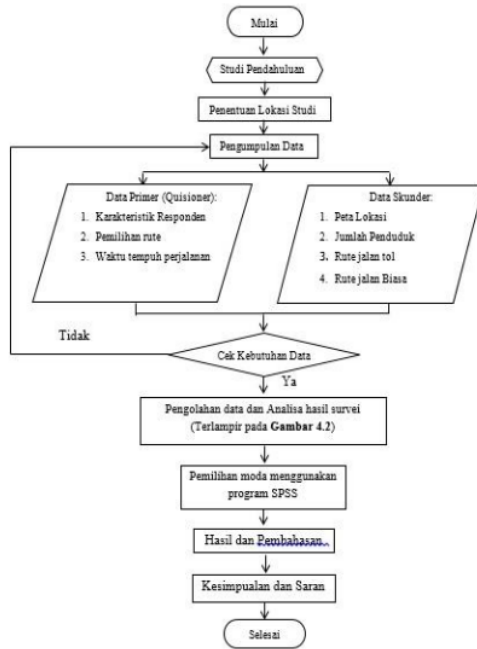
Gambar 2. Alur Penelitian
