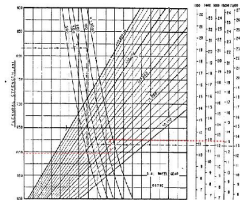
Gambar 1: Kurva perencanaan perkerasan rigid dual wheel
