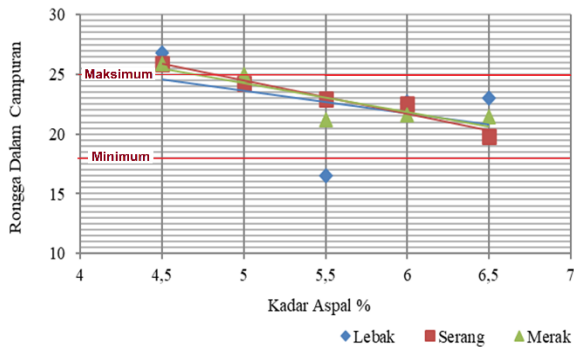
Gambar 7. Porosity
