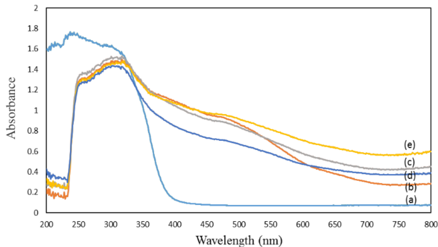
Figure 3. UV-Visible absorption spectra of the catalysts (a) \text{TiO}_2 (b) 10% Fe- \text{TiO}_2 , (c) 15% Fe- \text{TiO}_2 , (d) 20% Fe- \text{TiO}_2 , (e) Cu@Fe- \text{TiO}_2
