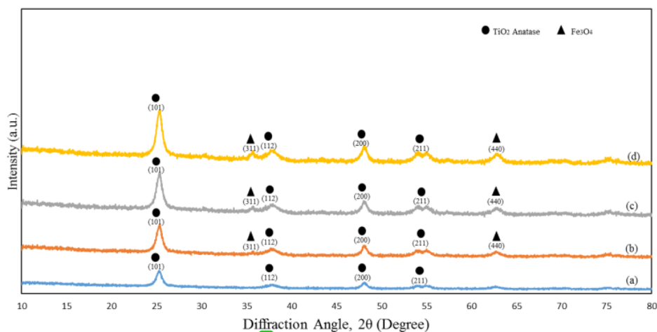
Figure 2. XRD Patterns of catalysts (a) \text{TiO}_2 , (b) 10% \text{Fe-TiO}_2 , (c) 15% \text{Fe-TiO}_2 , (d) 20% \text{Fe-TiO}_2 . Determination of particle size is done using the Debye-Scherrer equation as in equation (1).
