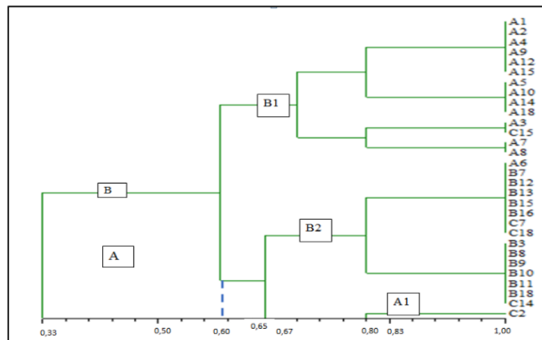
Figure 2. Result of Dendrogram Analysis
