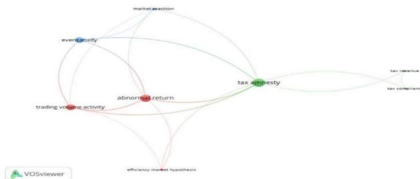
Figure 1. VOSViewer Output
