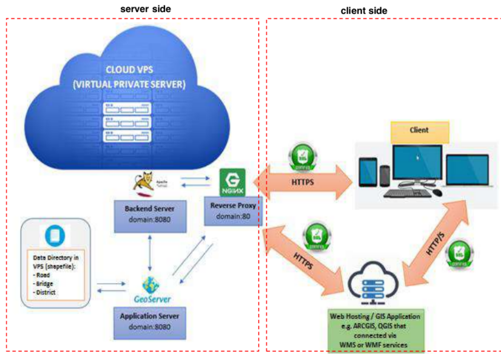
Figure 3. Multi-tier client/server architecture of the WebGIS.
