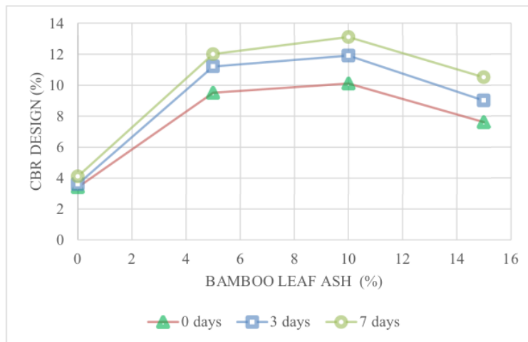
Figure 4. Relationship of CBR Value to Bamboo Leaf Ash Percentage
