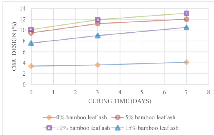
Figure 5. Relationship of CBR Value to Curing Time
