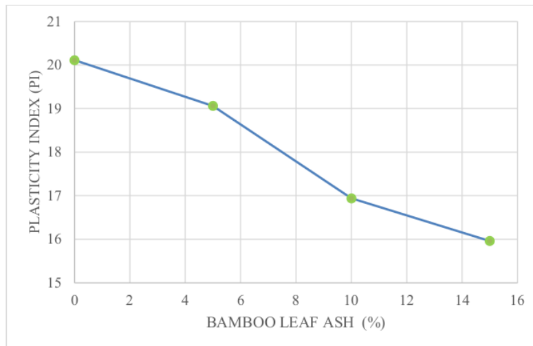
Figure 6. Relationship between Plasticity Index and Mixed Percentage
