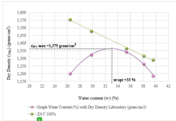
Figure 3. Relationship between soil dry density and water content
