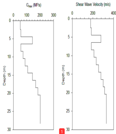
Fig. 8 One of display of shear modulus maximum ( G_{max} ) profile and shear wave velocity ( V_s ) profile from bedrock to surface
