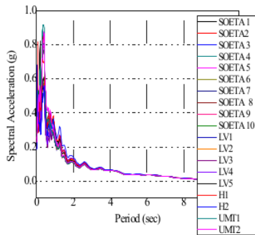
Fig.13 Response spectra using ground motion data of Borrego Mt 1968 earthquake event.
