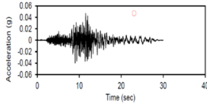
Fig.6 Ground motion display for Northridge-01 1994 earthquake Event
