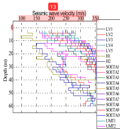
Fig.9 Shear wave velocity ( V_s ) profile for each point location study in Tangerang Region
