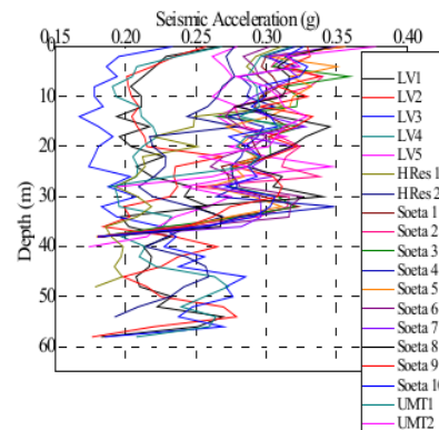
Fig.12 Profile of earthquake acceleration using ground motion data of Chichi Taiwan 1991 earthquake event
