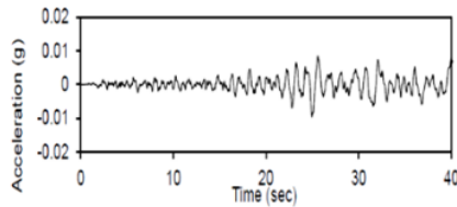
Fig.5 Ground motion display for Chichi Taiwan 1991 earthquake Event
