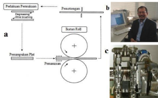
Figure 7. (a). Schematic of the Accumulative Roll Bonding (ARB) stage process (b). Nobuhiro Tsuji initiator of the ARB process (c). Rolling machine for ARB devices
