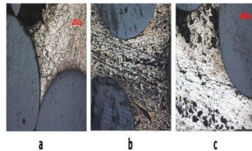
Gambar 7. Struktur Mikro Perbesaran 100x (a) Sampel annealing 1-siklus (b) Sampel annealing 2-siklus (c) Sampel annealing 3-siklus.
