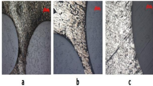
Gambar 6. Struktur mikro perbesaran 100x (a) sampel age hardening 1 siklus (b) sampel age hardening 2 siklus (c) sampel age hardening 3 siklus.
