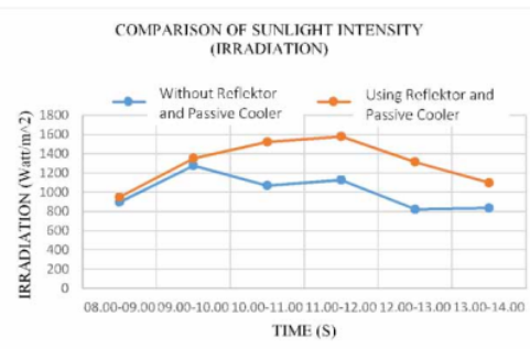
Figure 5. Comparison of the light intensity of solar panels without using reflectors and passive cooler with solar panels using reflectors and passive cooler
