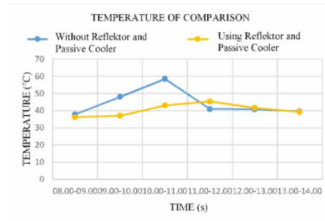
Figure 6. Comparison of temperature solar panels without using reflectors and passive cooler with solar panels using reflectors and passive cooler
