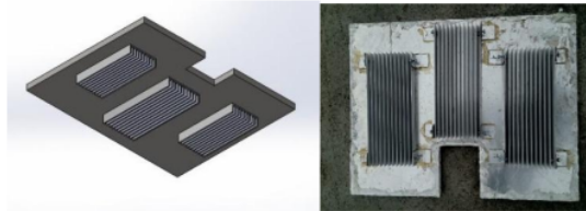
Figure 3. Passive Cooler Box and Heat Sink
