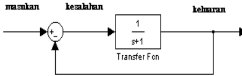
Gambar 6.4 Kesalahan Tunak 1/(s+1)
