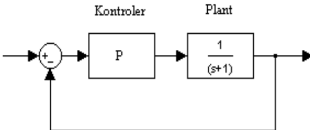
Gambar 8.1 Kontroler Proportional
