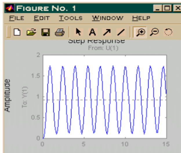
Gambar 9.19 Respon Step Sistem K=126 (batas kestabilan)
