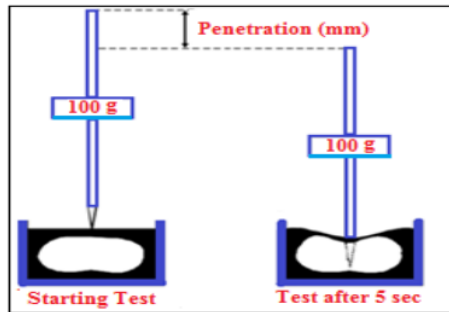
Figure 5. Schematic view of penetration test.
