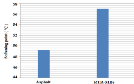
Figure 9. Results of softening point test.
