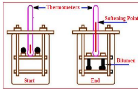
Figure 6. Schematic view of softening point test.
