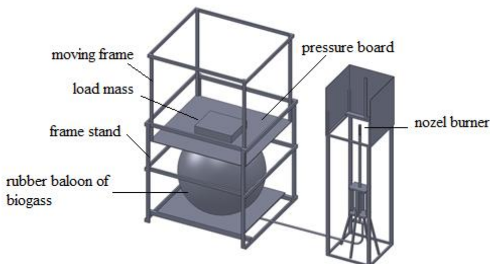
Figure 1. Skecth of flame measuring instrument.
